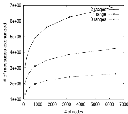
Fig. 4. Scalability in the number of nodes with range queries. 40000 subscriptions, 40000 publications
